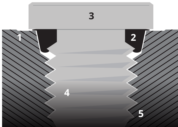
O-Ring Boss Plug SAE J1926 or ISO 6149 Ports
